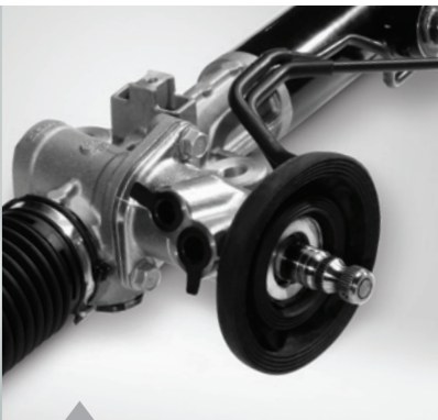
RACK & PINION
